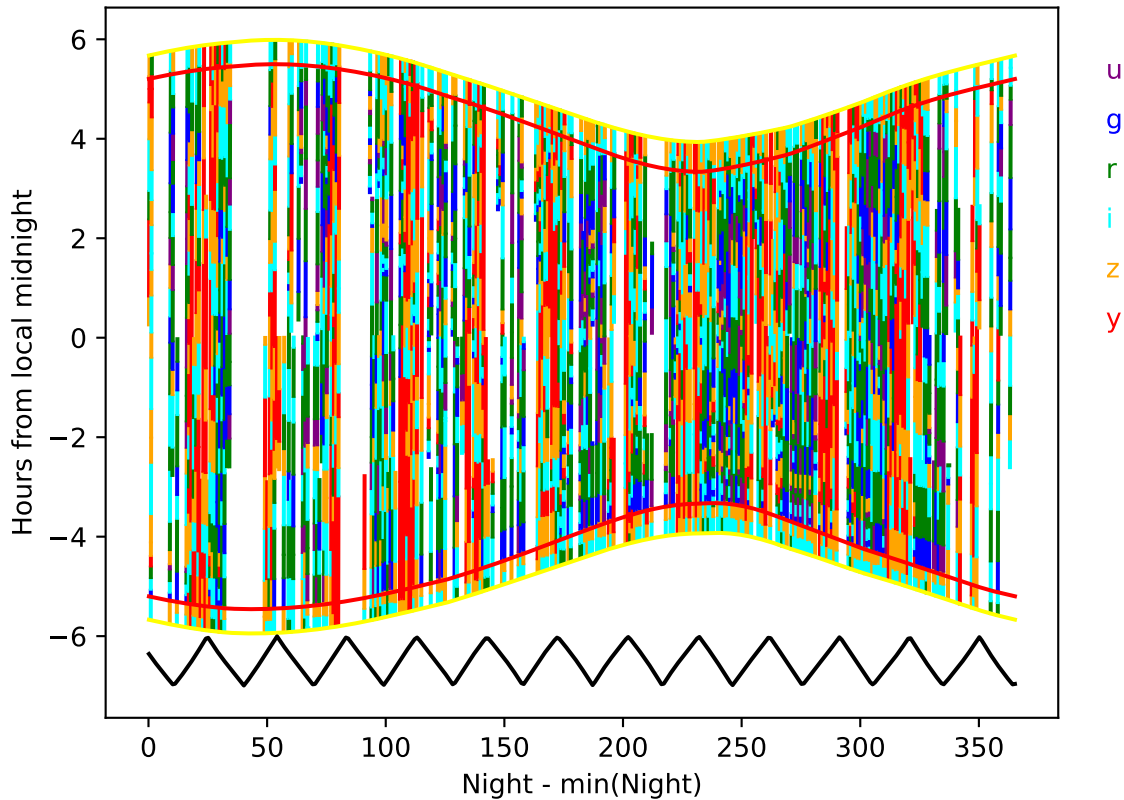
ddf_acor_sf20_lsf0_lsr0_v3.4_10yrs year 4-5: Hourglass
