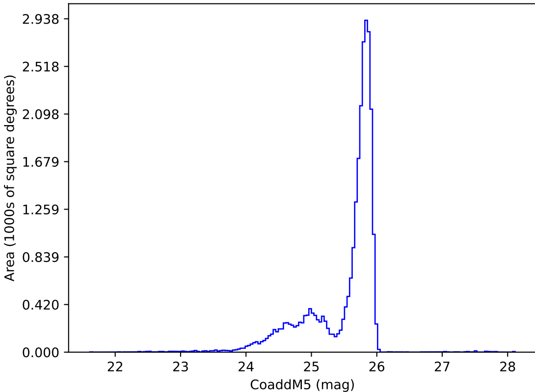
ddf_acor_sf20_lsf0_lsr0_v3.4_10yrs z: CoaddM5
