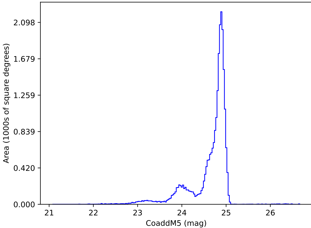
ddf_acor_sf20_lsf0_lsr0_v3.4_10yrs y: CoaddM5
