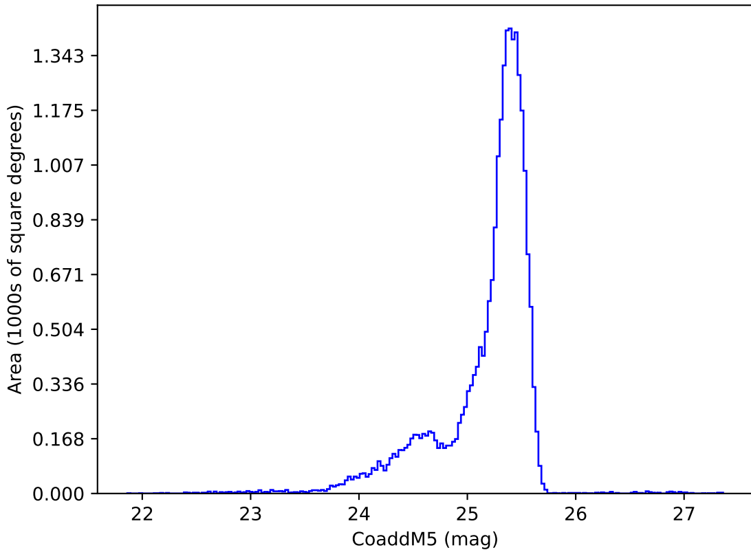
ddf_acor_sf20_lsf0_lsr0_v3.4_10yrs u: CoaddM5
