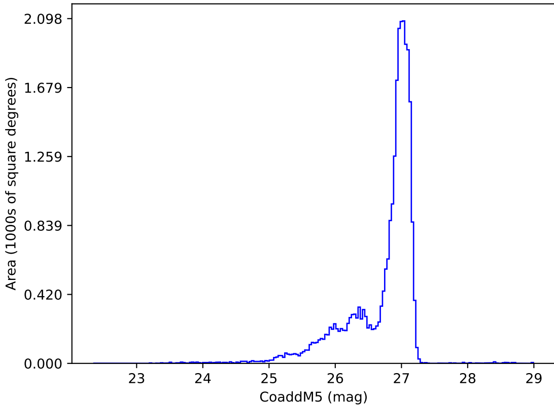
ddf_acor_sf20_lsf0_lsr0_v3.4_10yrs r: CoaddM5
