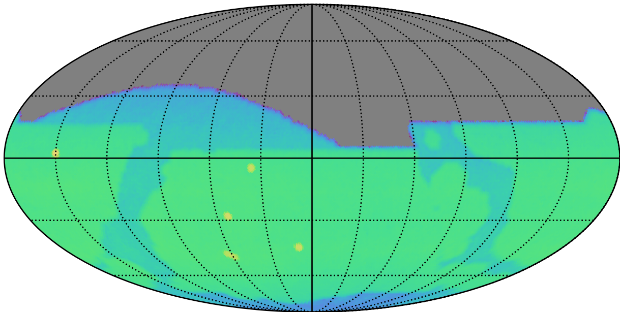
ddf_acor_sf20_lsf0_lsr0_v3.4_10yrs i: CoaddM5
