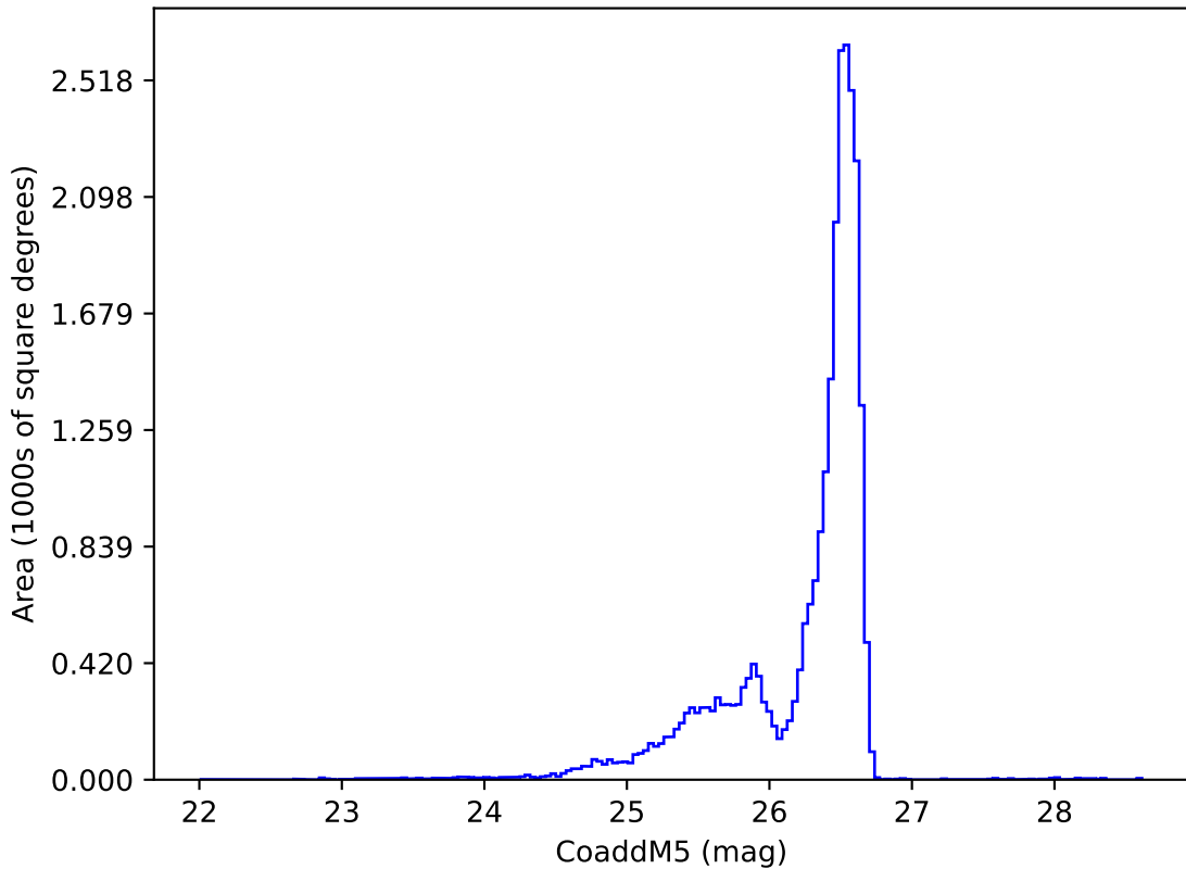
ddf_acor_sf20_lsf0_lsr0_v3.4_10yrs i: CoaddM5
