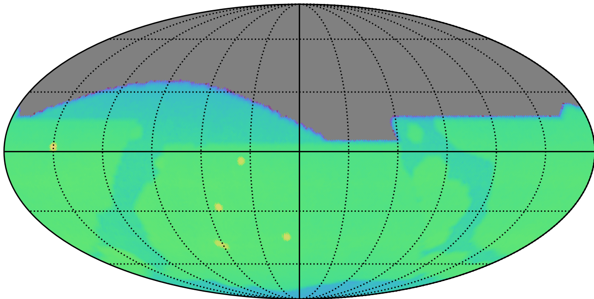
ddf_acor_sf20_lsf0_lsr0_v3.4_10yrs : CoaddM5
