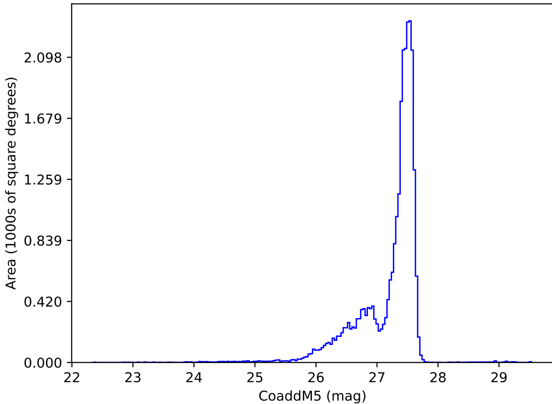
ddf_acor_sf20_lsf0_lsr0_v3.4_10yrs : CoaddM5
