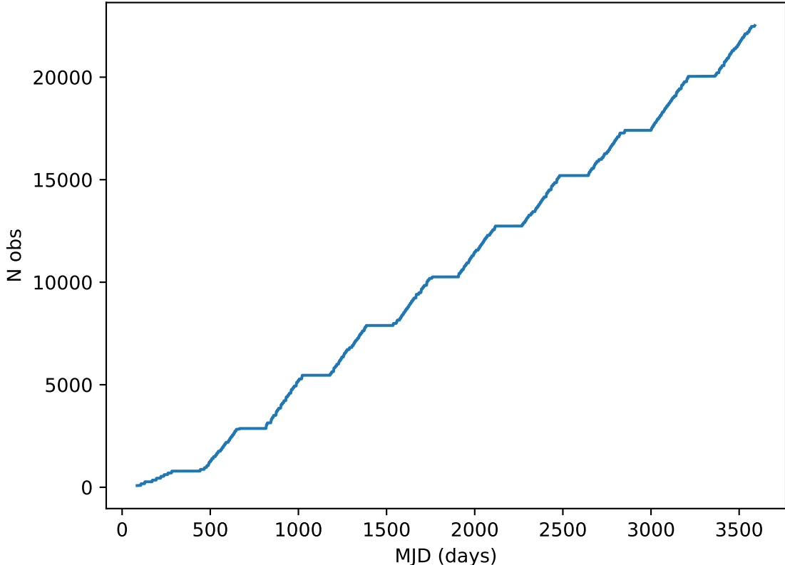
ddf_acor_sf20_lsf0_lsr0_v3.4_10yrs all bands: DD:XMM_LSS Cumulative NVisits
