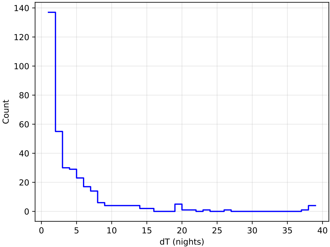
ddf_acor_sf20_lsf0_lsr0_v3.4_10yrs all bands: DD:WFD Delta Nights Histogram
