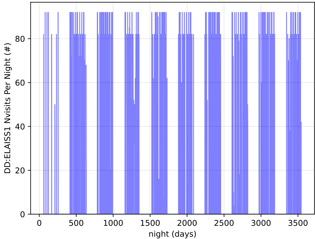
ddf_acor_sf20_lsf0_lsr0_v3.4_10yrs all bands: DD:ELAISS1 Nvisits Per Night
