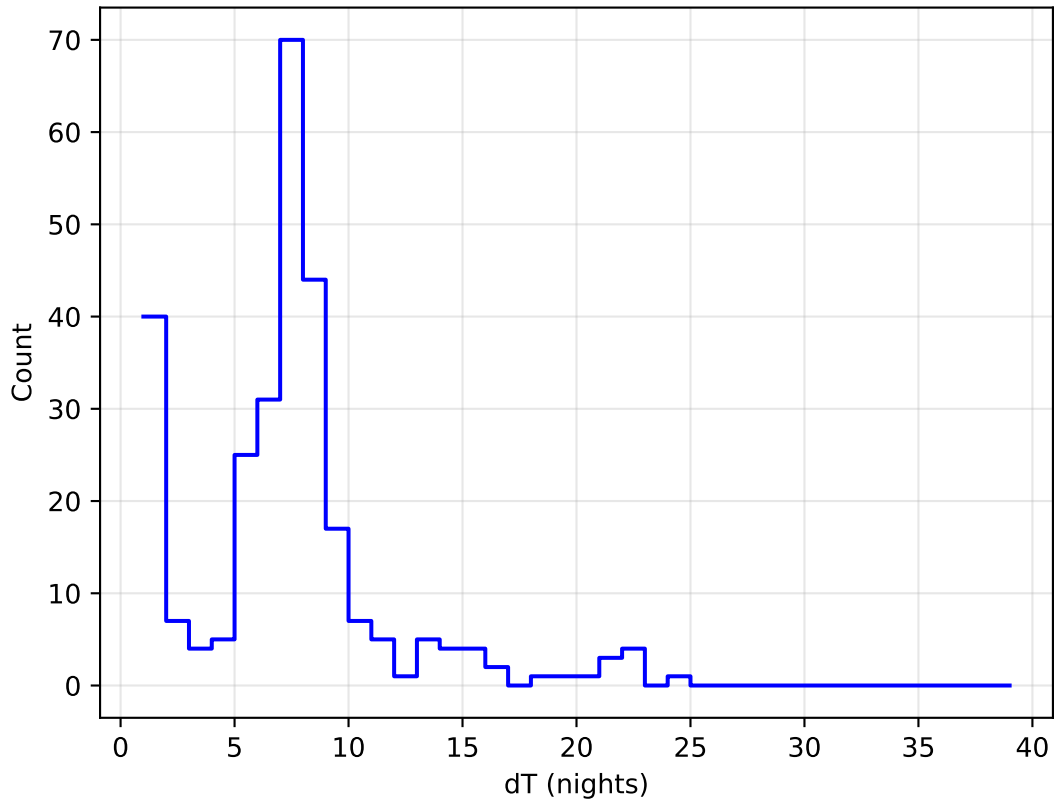
ddf_acor_sf20_Isf0_Isr0_v3.4_10yrs all bands: DD:ELAISS1 Delta Nights Histogram
