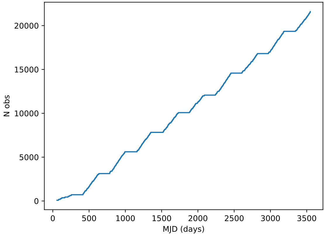
ddf_acor_sf20_lsf0_lsr0_v3.4_10yrs all bands: DD:ELAISS1 Cumulative NVisits
