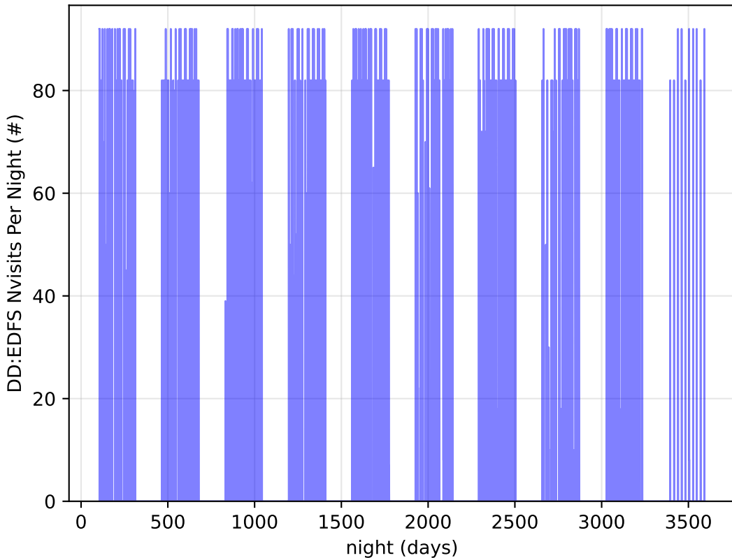
ddf_acor_sf20_lsf0_lsr0_v3.4_10yrs all bands: DD:EDFS Nvisits Per Night
