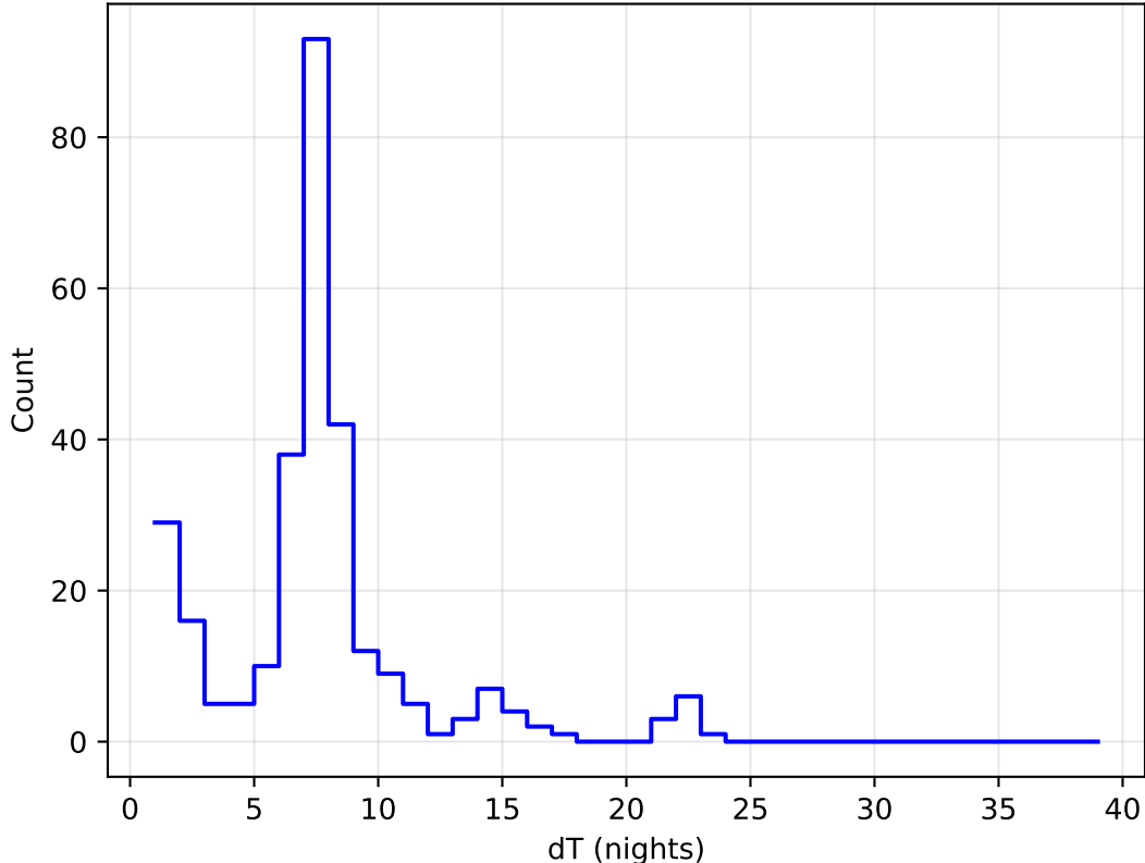
ddf_acor_sf20_lsf0_lsr0_v3.4_10yrs all bands: DD:EDFS Delta Nights Histogram
