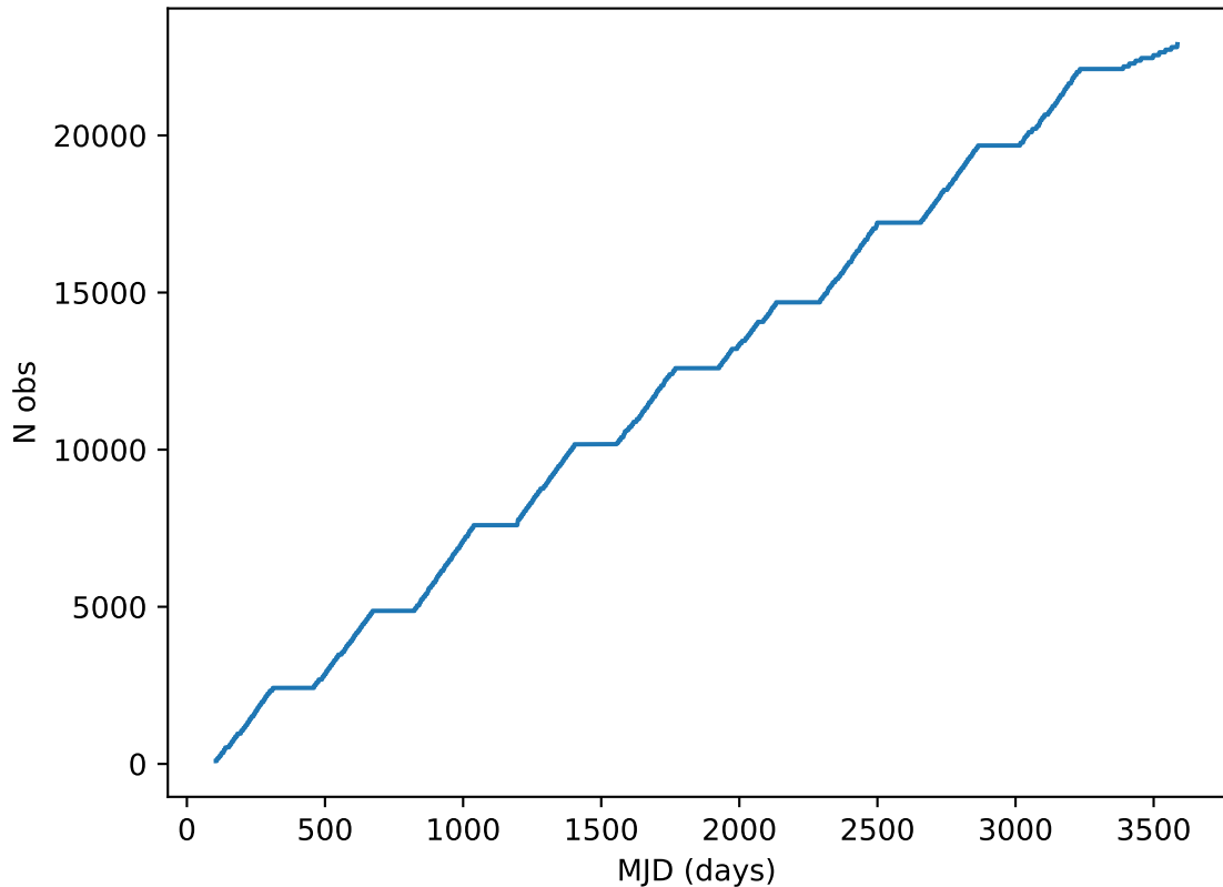
ddf_acor_sf20_lsf0_lsr0_v3.4_10yrs all bands: DD:ECDFS Cumulative NVisits
