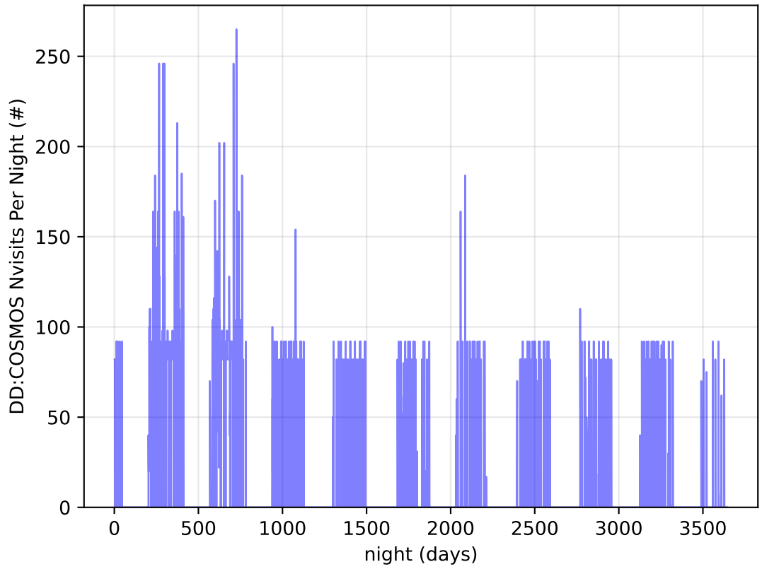
ddf_acor_sf20_lsf0_lsr0_v3.4_10yrs all bands: DD: COSMOS Nvisits Per Night
