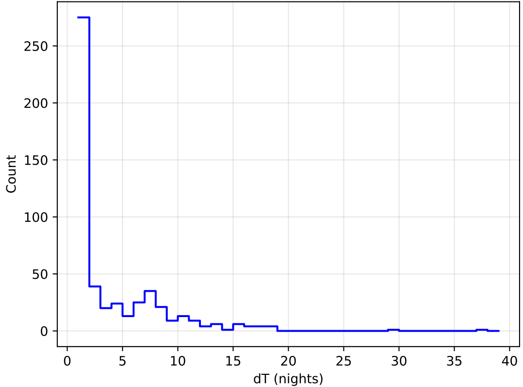
ddf_acor_sf20_lsf0_lsr0_v3.4_10yrs all bands: DD: COSMOS Delta Nights Histogram
