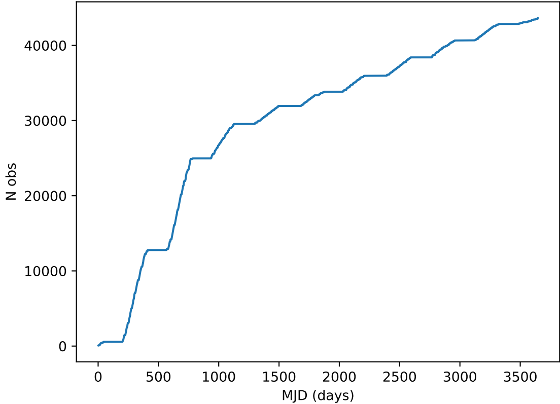
ddf_acor_sf20_lsf0_lsr0_v3.4_10yrs all bands: DD: COSMOS Cumulative NVisits
