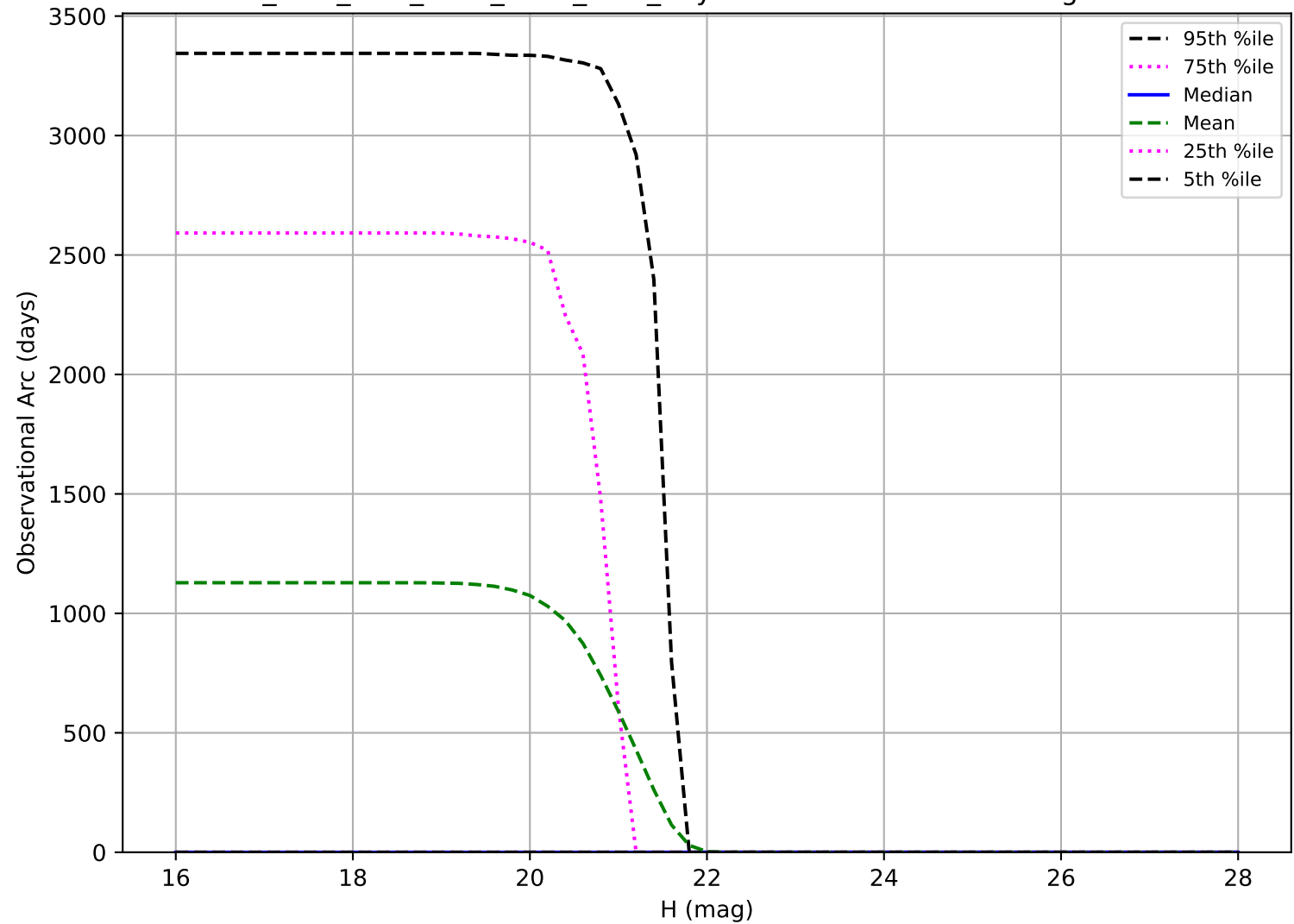
ddf_acor_sf15_lsf40_lsr50_v3.4_10yrs: Observational Arc Length Vatira
