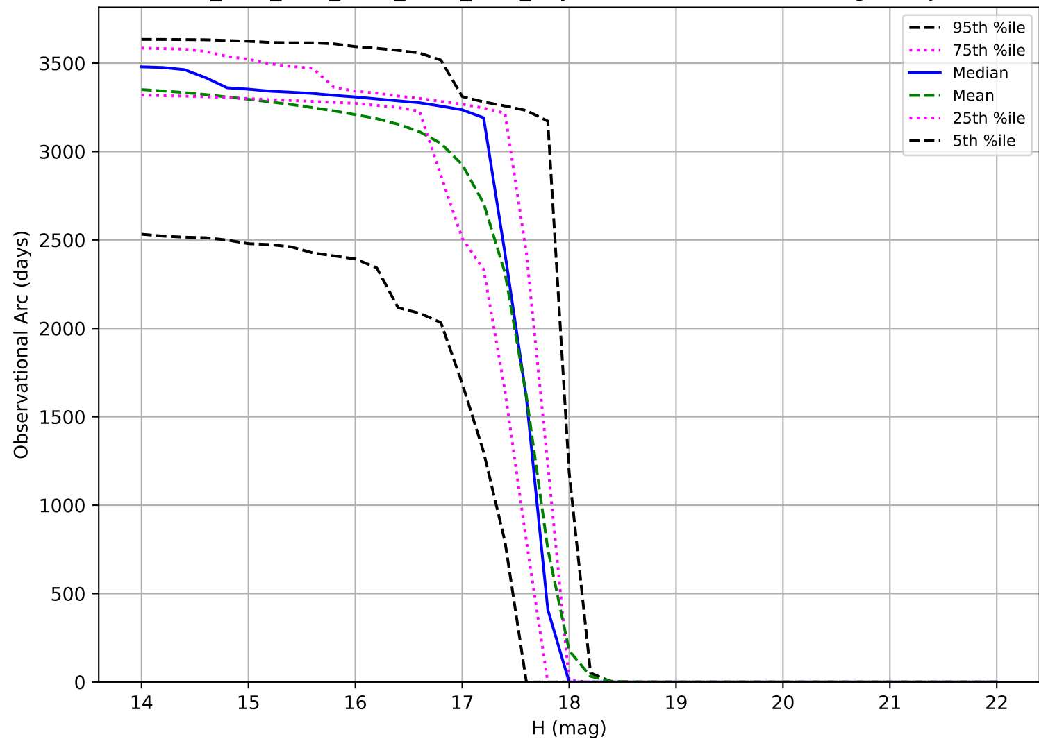
ddf_acor_sf15_lsf40_lsr50_v3.4_10yrs: Observational Arc Length Trojan
