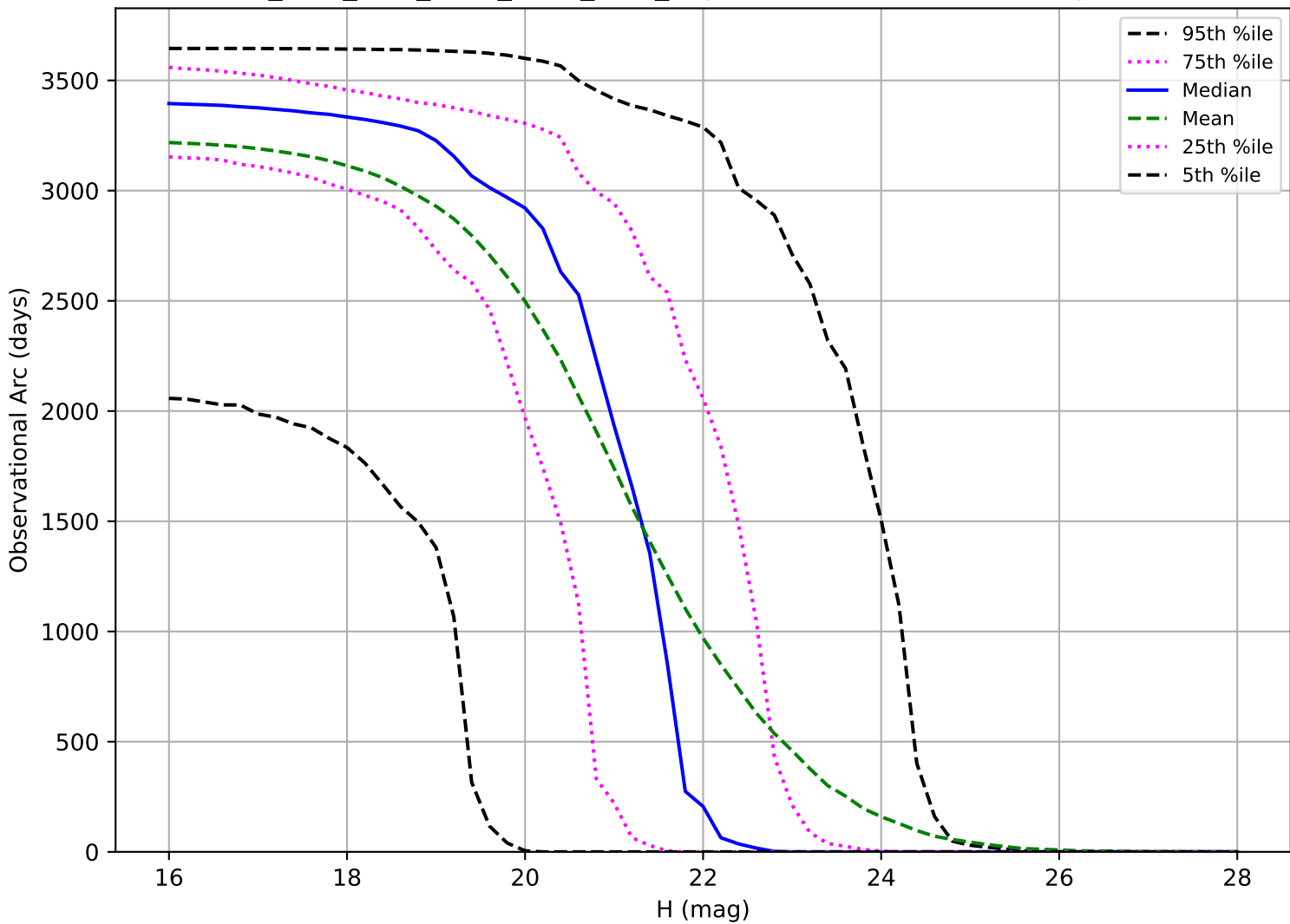
ddf_acor_sf15_lsf40_lsr50_v3.4_10yrs: Observational Arc Length PHA
