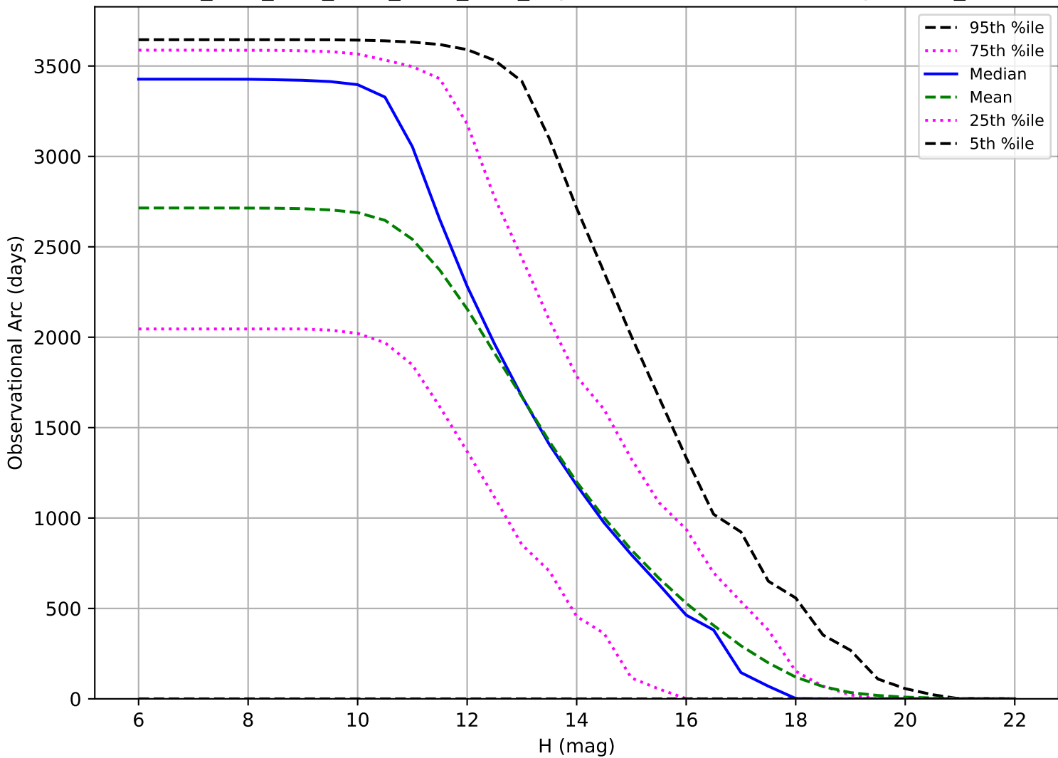
ddf_acor_sf15_lsf40_lsr50_v3.4_10yrs: Observational Arc Length OCC_r5
