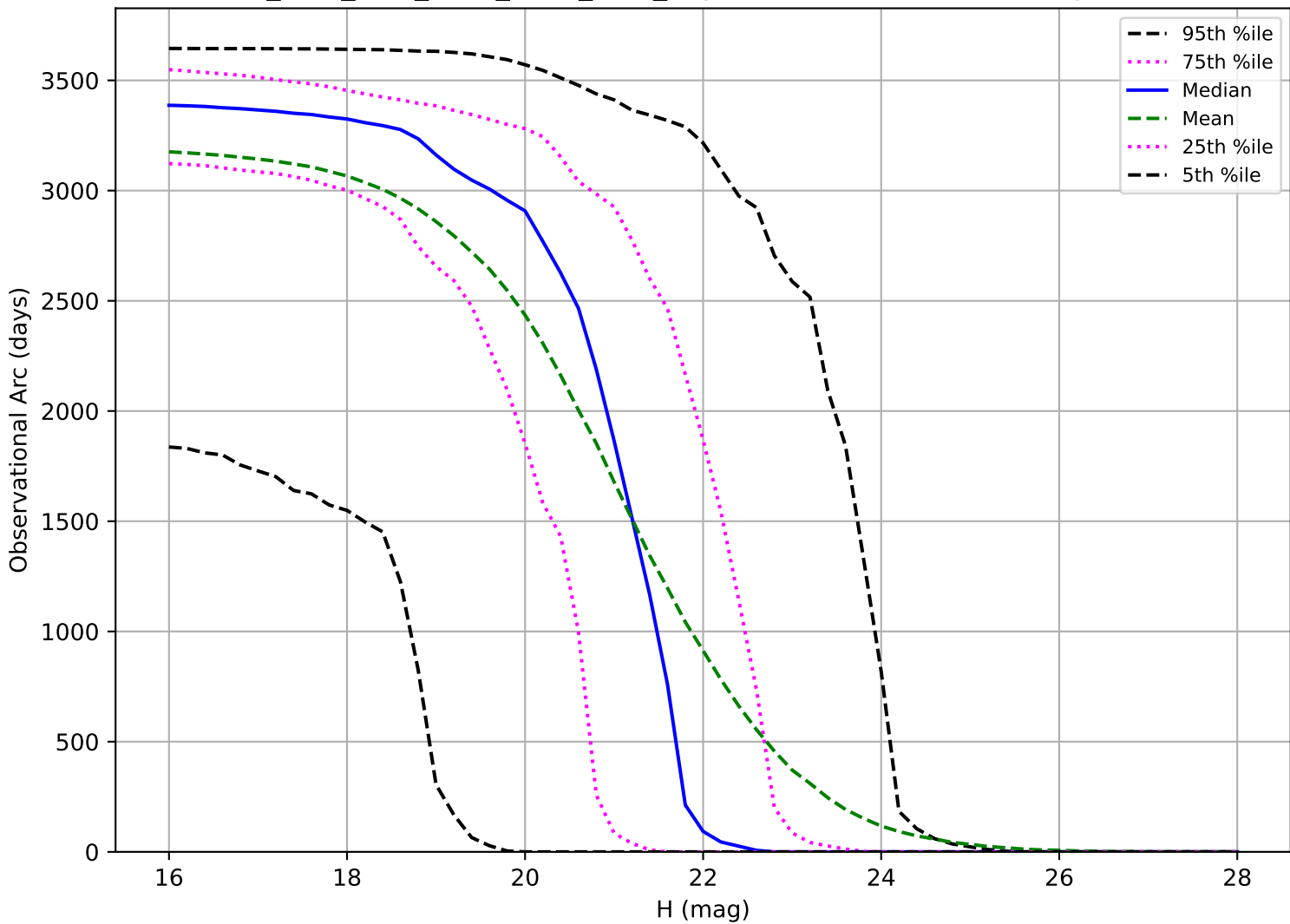
ddf_acor_sf15_lsf40_lsr50_v3.4_10yrs: Observational Arc Length NEO
