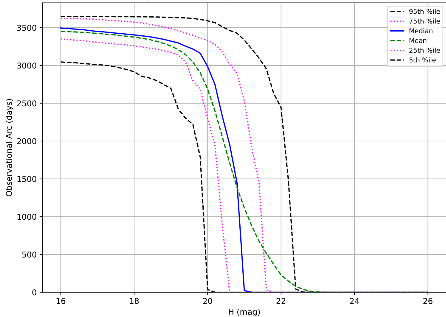
ddf_acor_sf15_lsf40_lsr50_v3.4_10yrs: Observational Arc Length MBA
