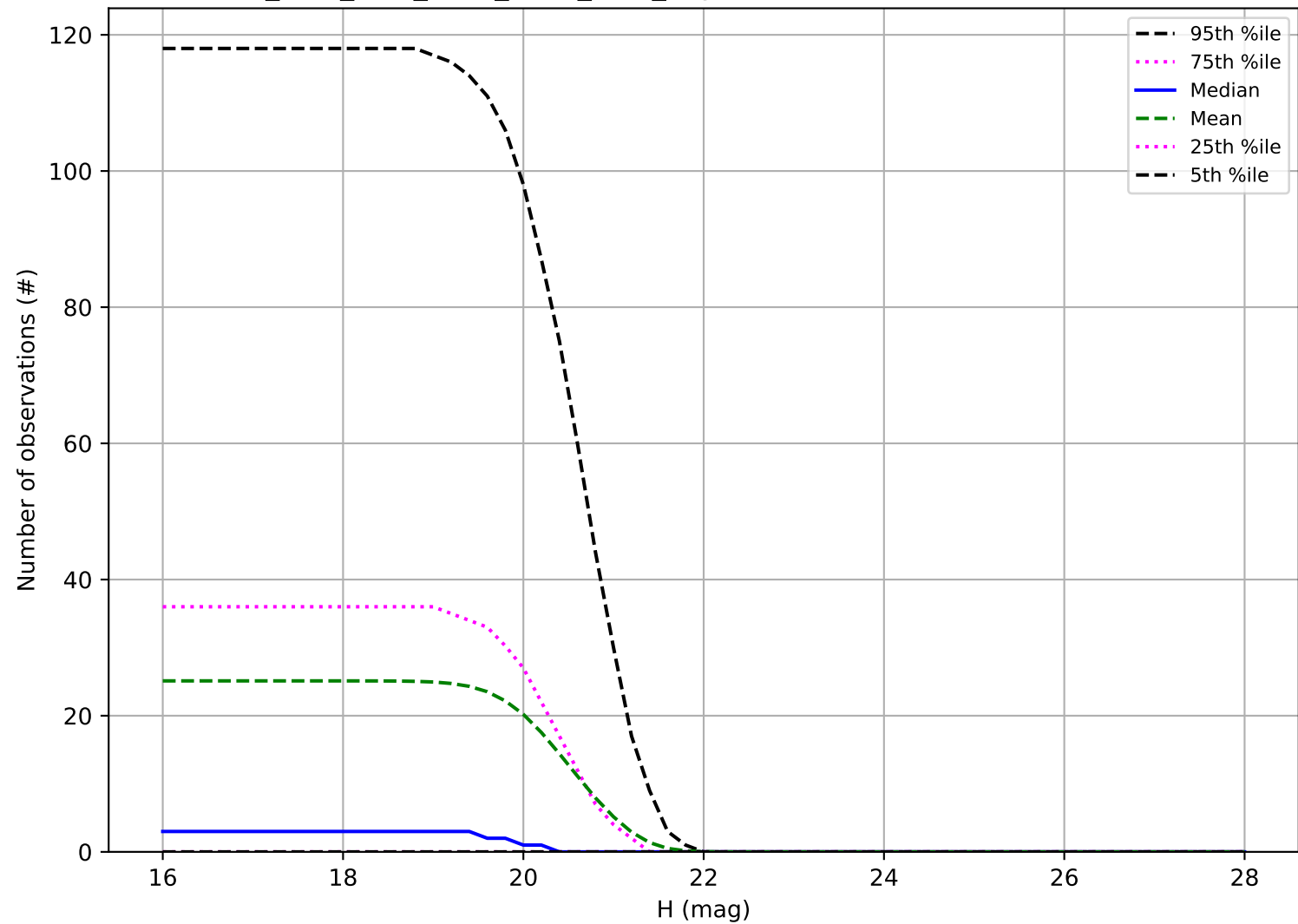
ddf_acor_sf15_lsf40_lsr50_v3.4_10yrs: Number of observations Vatira
