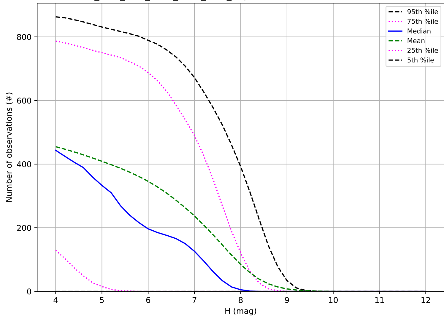
ddf_acor_sf15_lsf40_lsr50_v3.4_10yrs: Number of observations TNO
