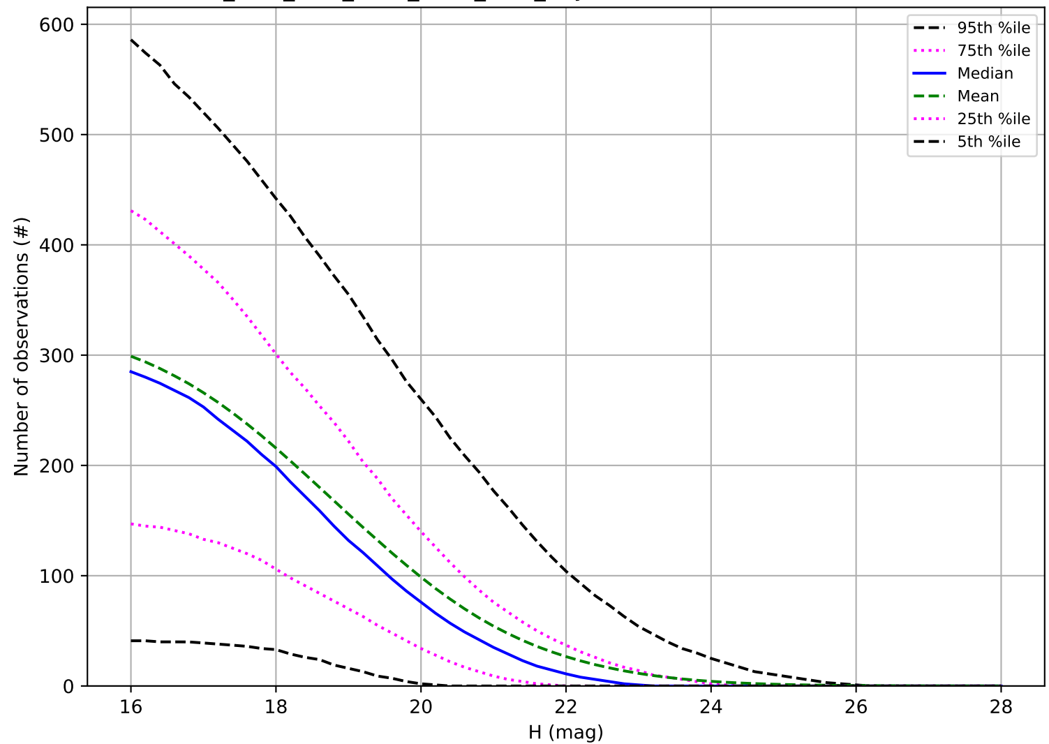
ddf_acor_sf15_lsf40_lsr50_v3.4_10yrs: Number of observations PHA
