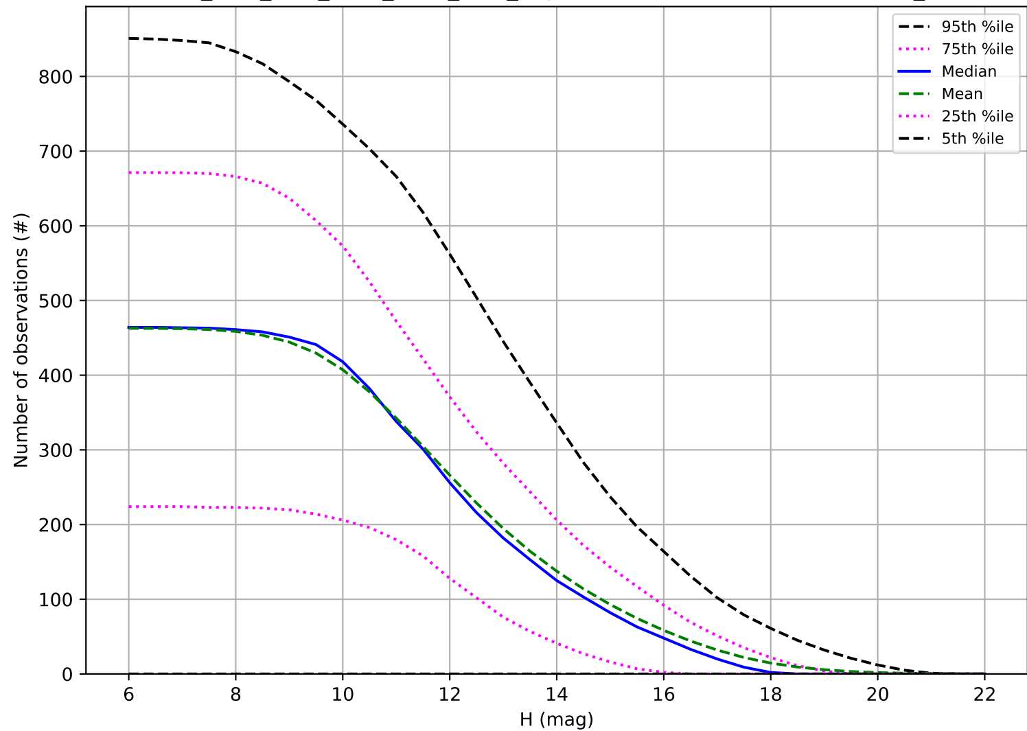
ddf_acor_sf15_lsf40_lsr50_v3.4_10yrs: Number of observations OCC_r5
