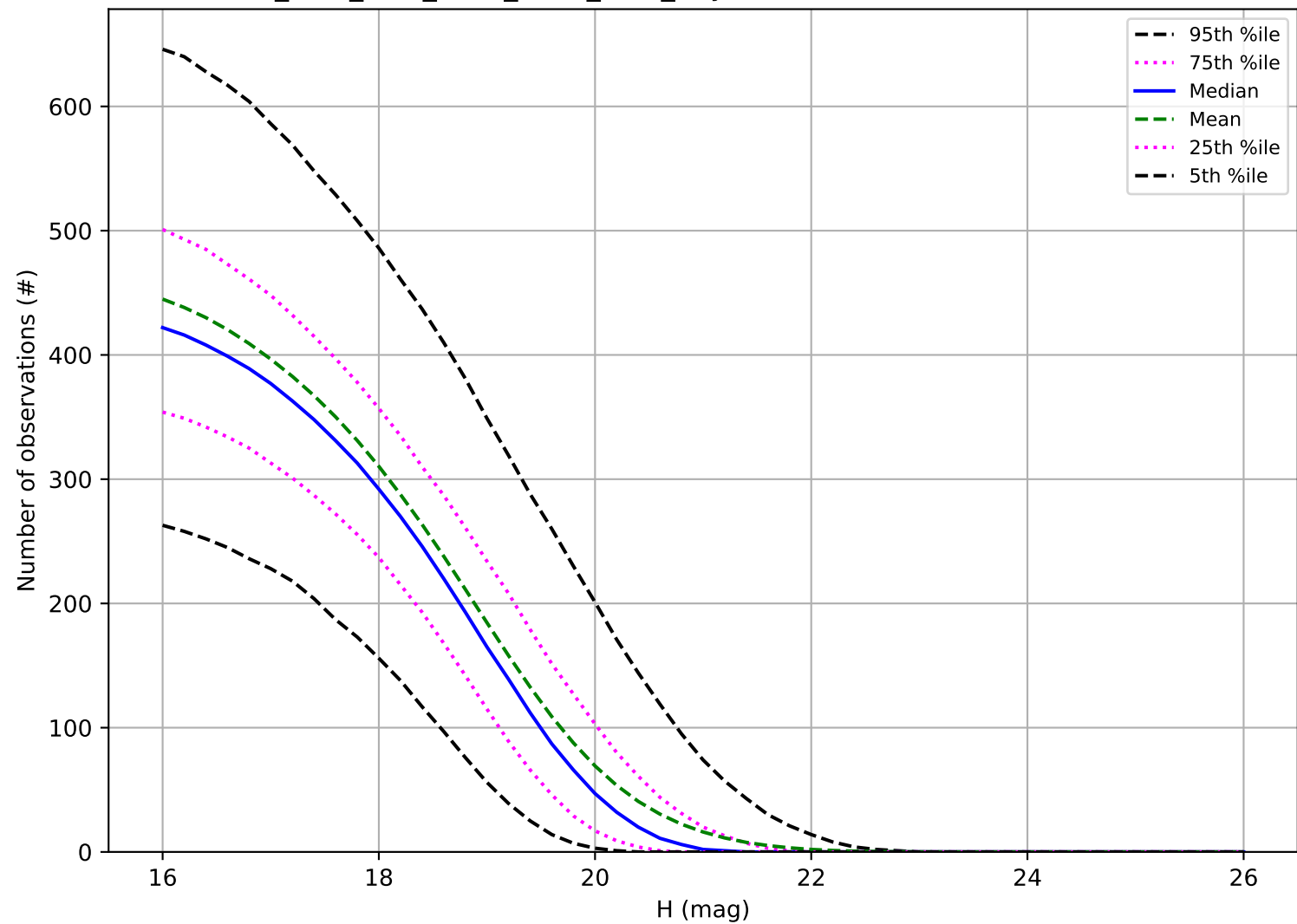
ddf_acor_sf15_Isf40_Isr50_v3.4_10yrs: Number of observations MBA
