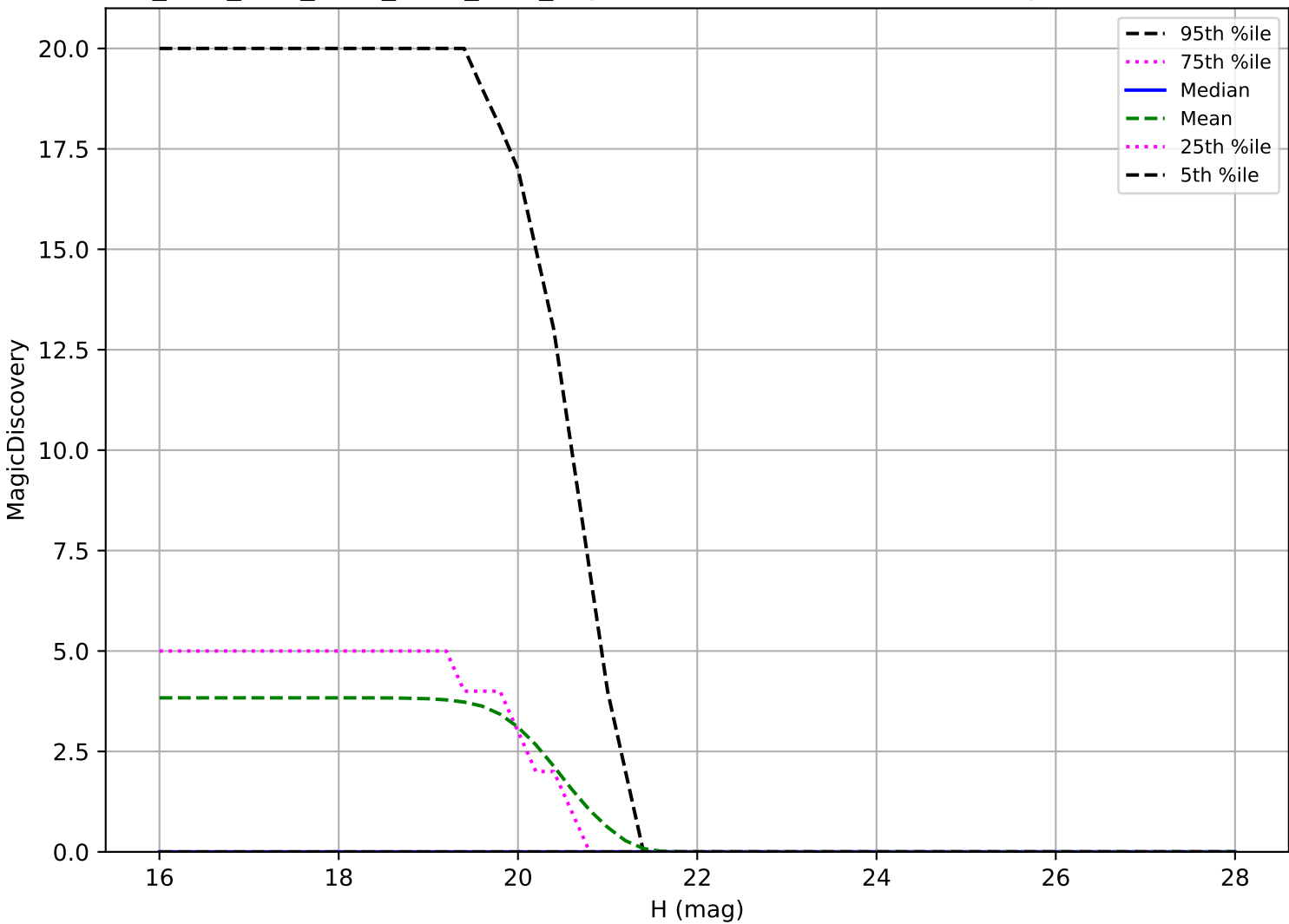
ddf_acor_sf15_lsf40_lsr50_v3.4_10yrs: Vatira 6 detections in 60 nights detection loss
