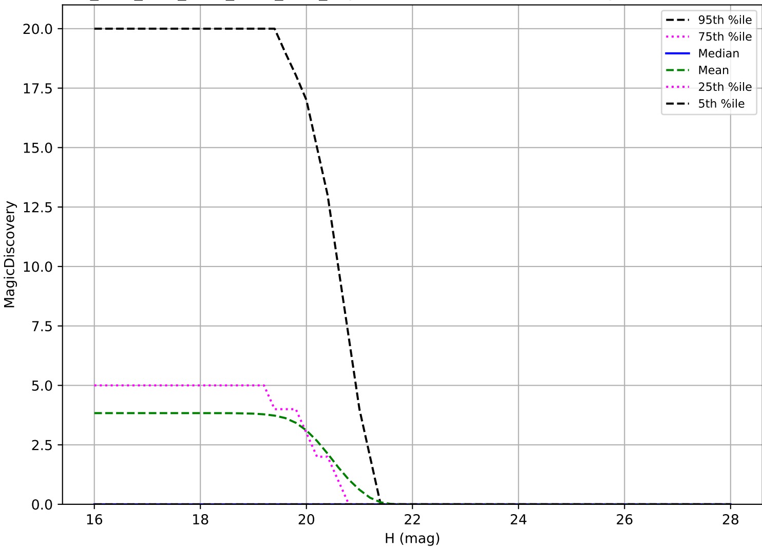
ddf_acor_sf15_lsf40_lsr50_v3.4_10yrs: Vatra 6 detections in 60 nights detection loss
