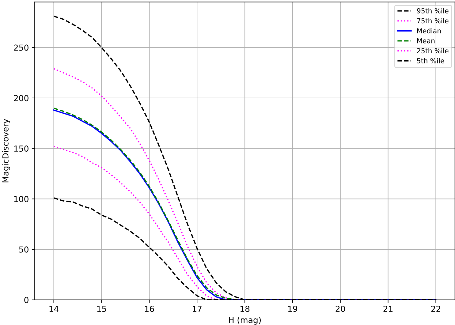
ddf_acor_sf15_lsf40_lsr50_v3.4_10yrs: Trojan 6 detections in 60 nights detection loss
