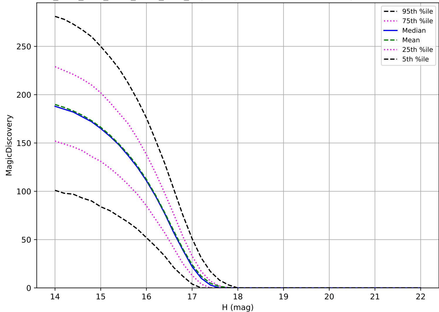
ddf_acor_sf15_lsf40_lsr50_v3.4_10yrs: Trojan 6 detections in 60 nights detection loss
