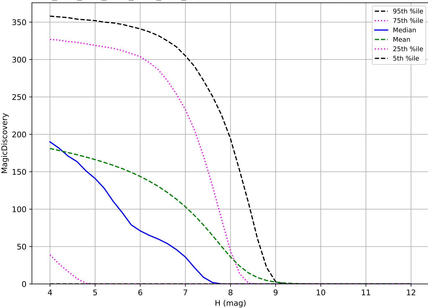
ddf_acor_sf15_lsf40_lsr50_v3.4_10yrs: TNO 6 detections in 60 nights detection loss
