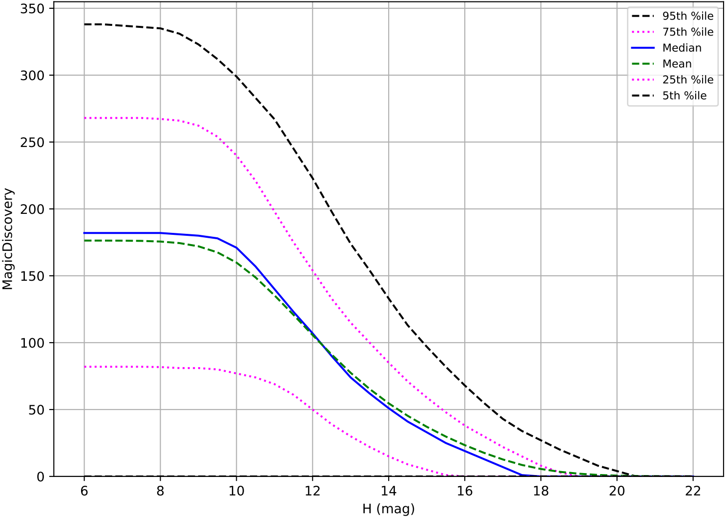
ddf_acor_sf15_lsf40_lsr50_v3.4_10yrs: OCC_r5 6 detections in 60 nights detection loss
