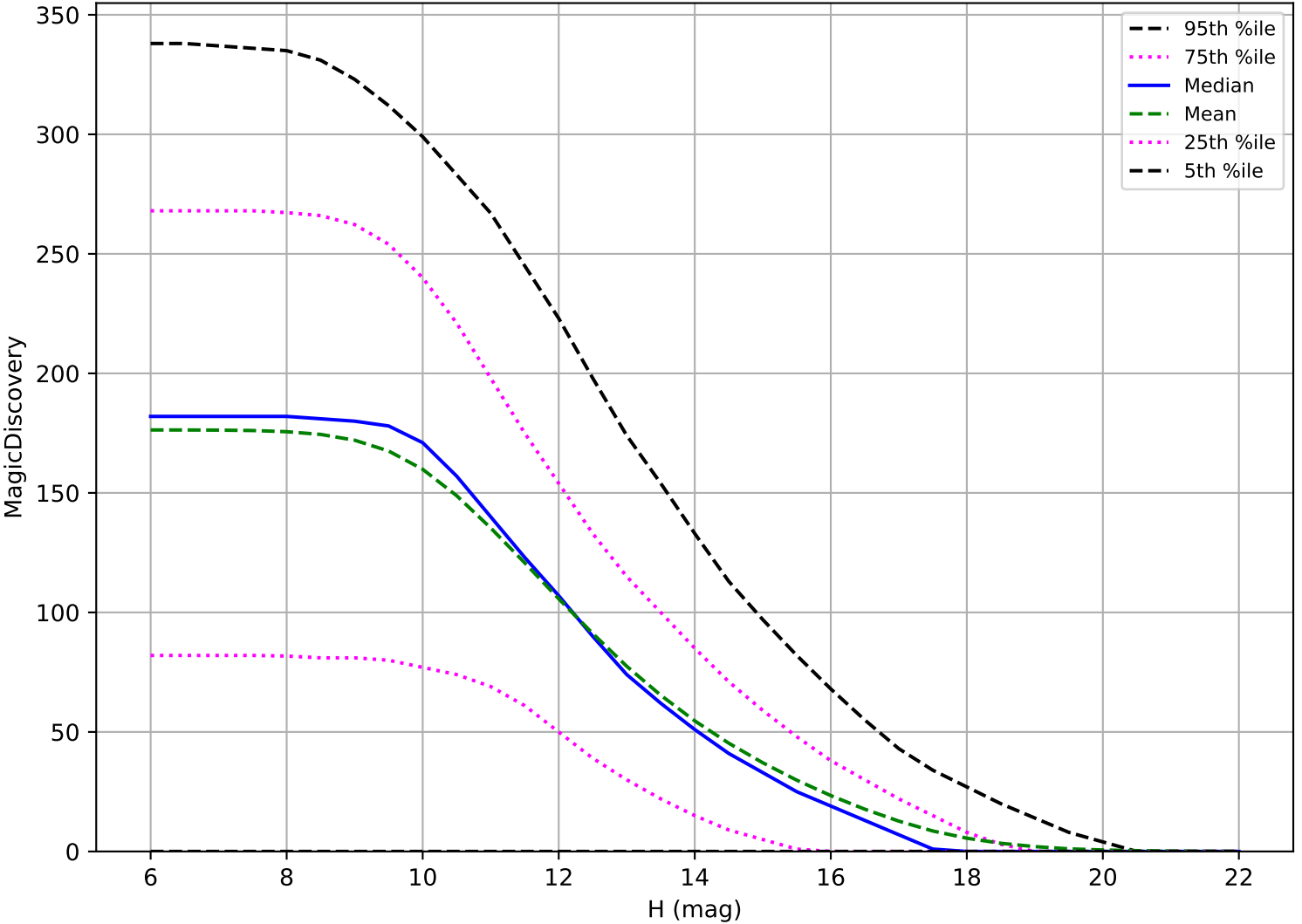
ddf_acor_sf15_lsf40_lsr50_v3.4_10yrs: OCC_r5 6 detections in 60 nights detection loss
