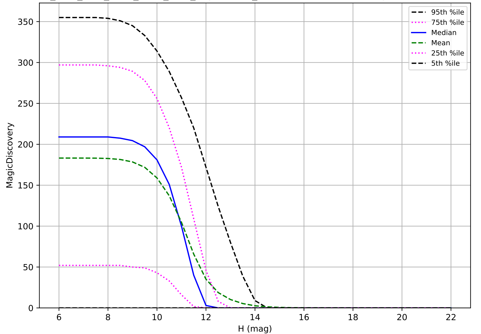
ddf_acor_sf15_lsf40_lsr50_v3.4_10yrs: OCC_r20 6 detections in 60 nights detection loss
