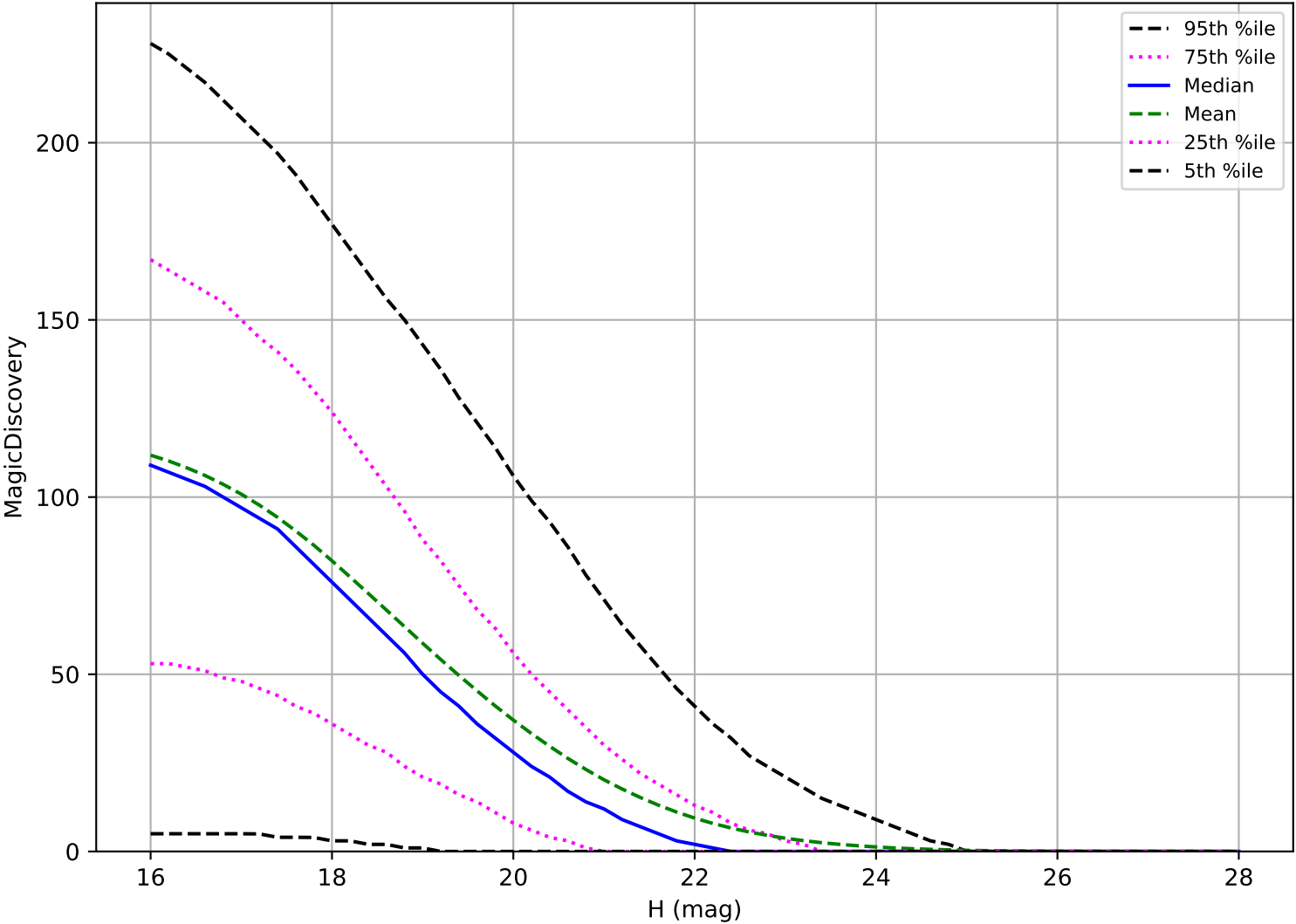
ddf_acor_sf15_lsf40_lsr50_v3.4_10yrs: NEO 6 detections in 60 nights detection loss
