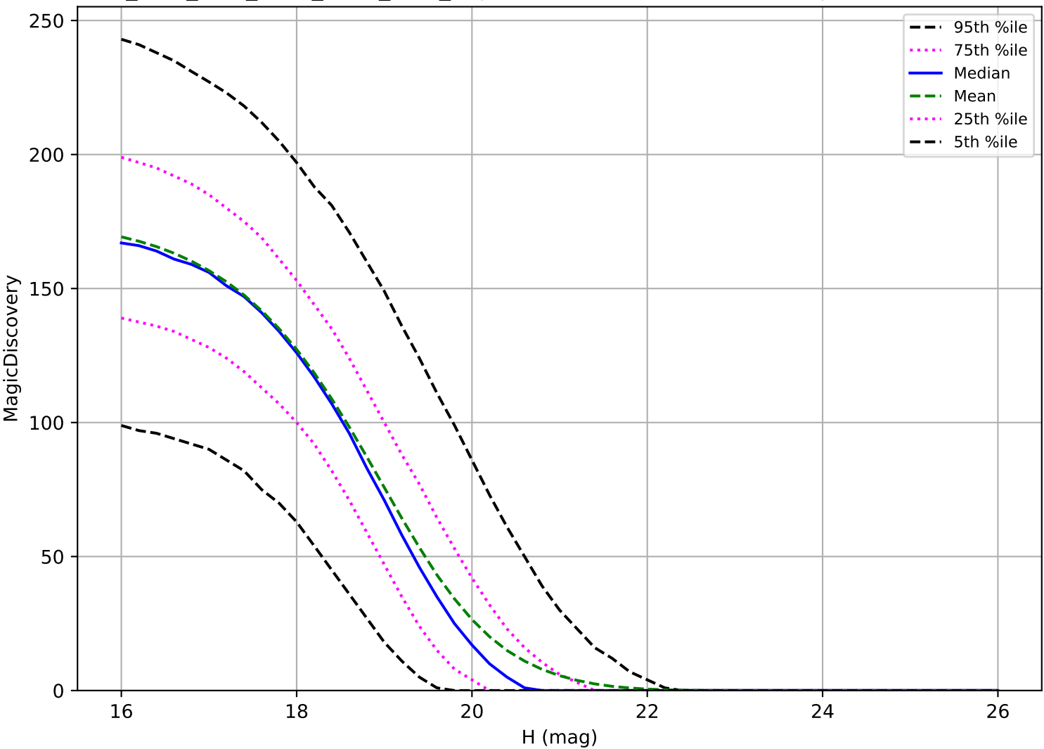
ddf_acor_sf15_lsf40_lsr50_v3.4_10yrs: MBA 6 detections in 60 nights detection loss
