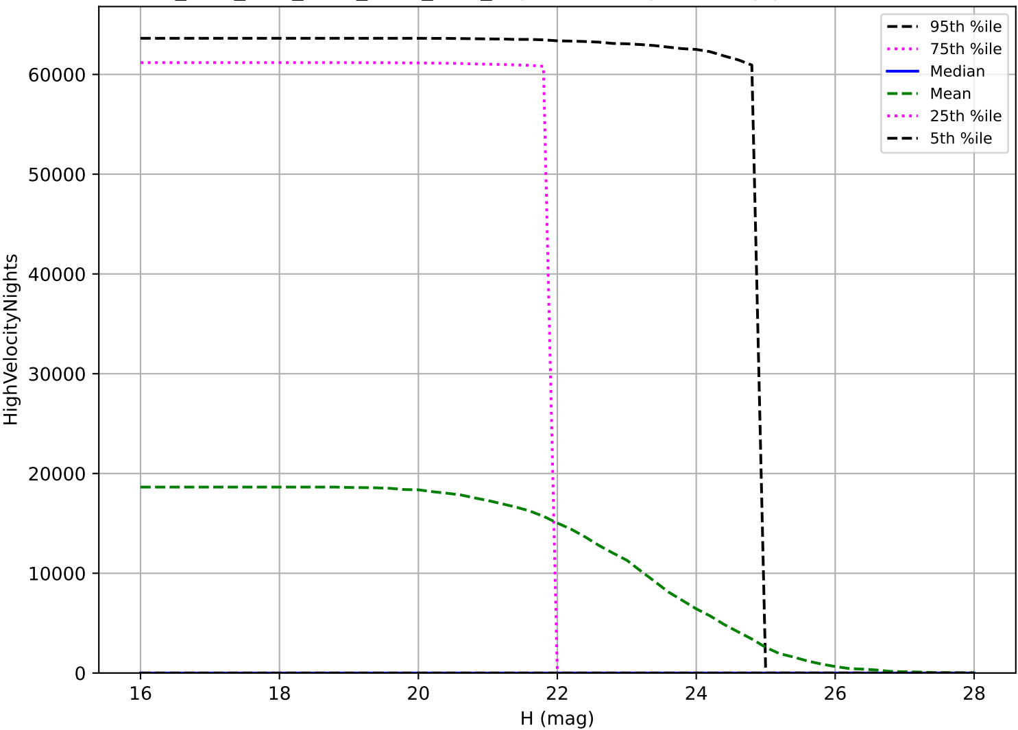
ddf_acor_sf15_lsf40_lsr50_v3.4_10yrs: NEO High velocity pair detection loss
