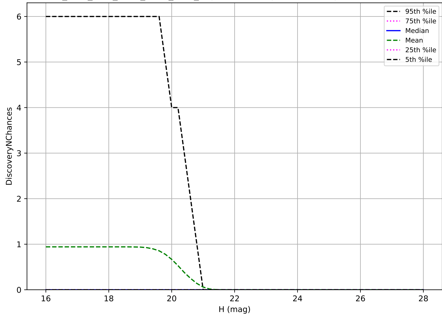
ddf_acor_sf15_lsf40_lsr50_v3.4_10yrs: Vatira 3 pairs in 15 nights detection loss
