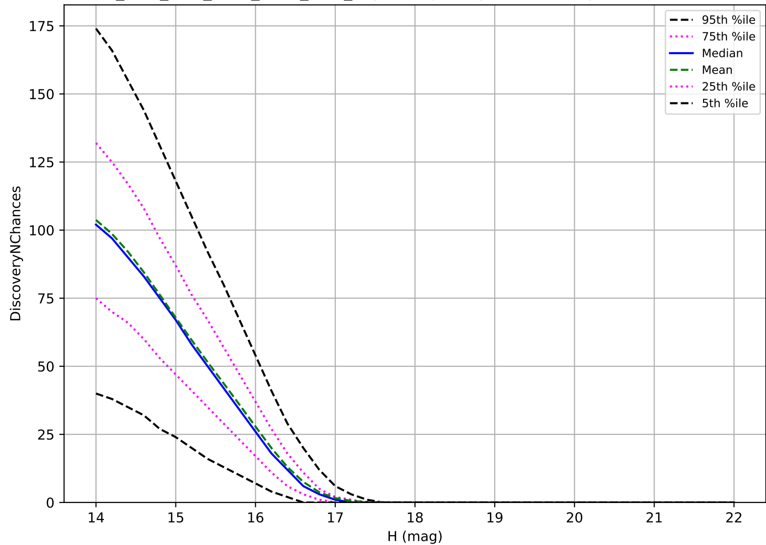
ddf_acor_sf15_lsf40_lsr50_v3.4_10yrs: Trojan 3 pairs in 15 nights detection loss
