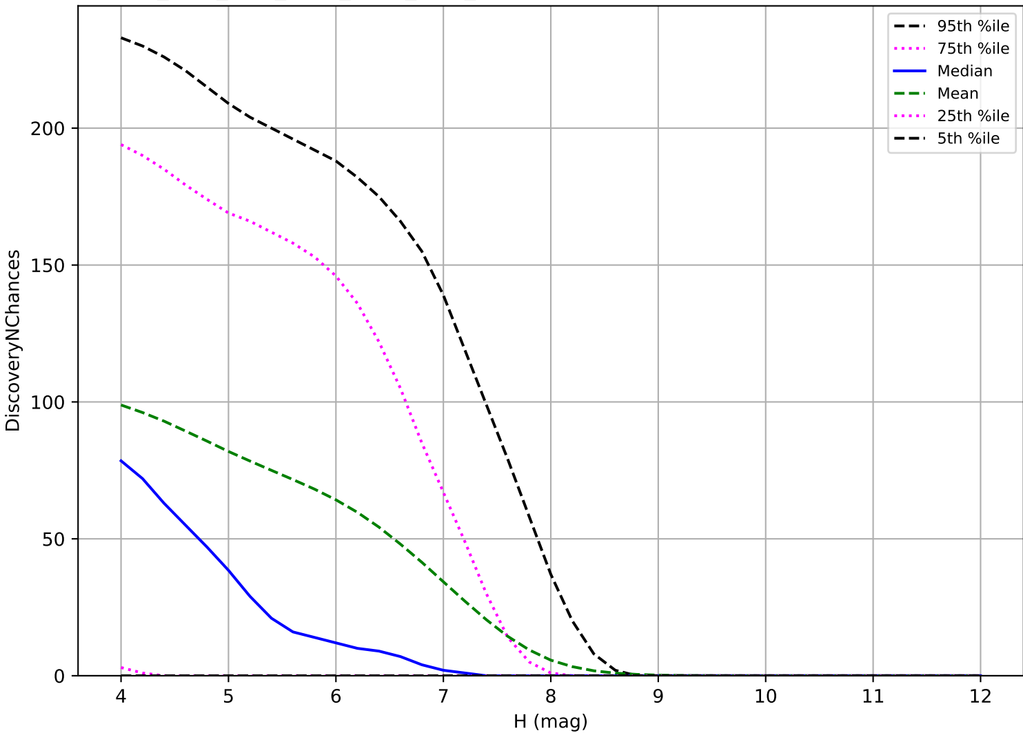
ddf_acor_sf15_lsf40_lsr50_v3.4_10yrs: TNO 3 pairs in 15 nights detection loss
