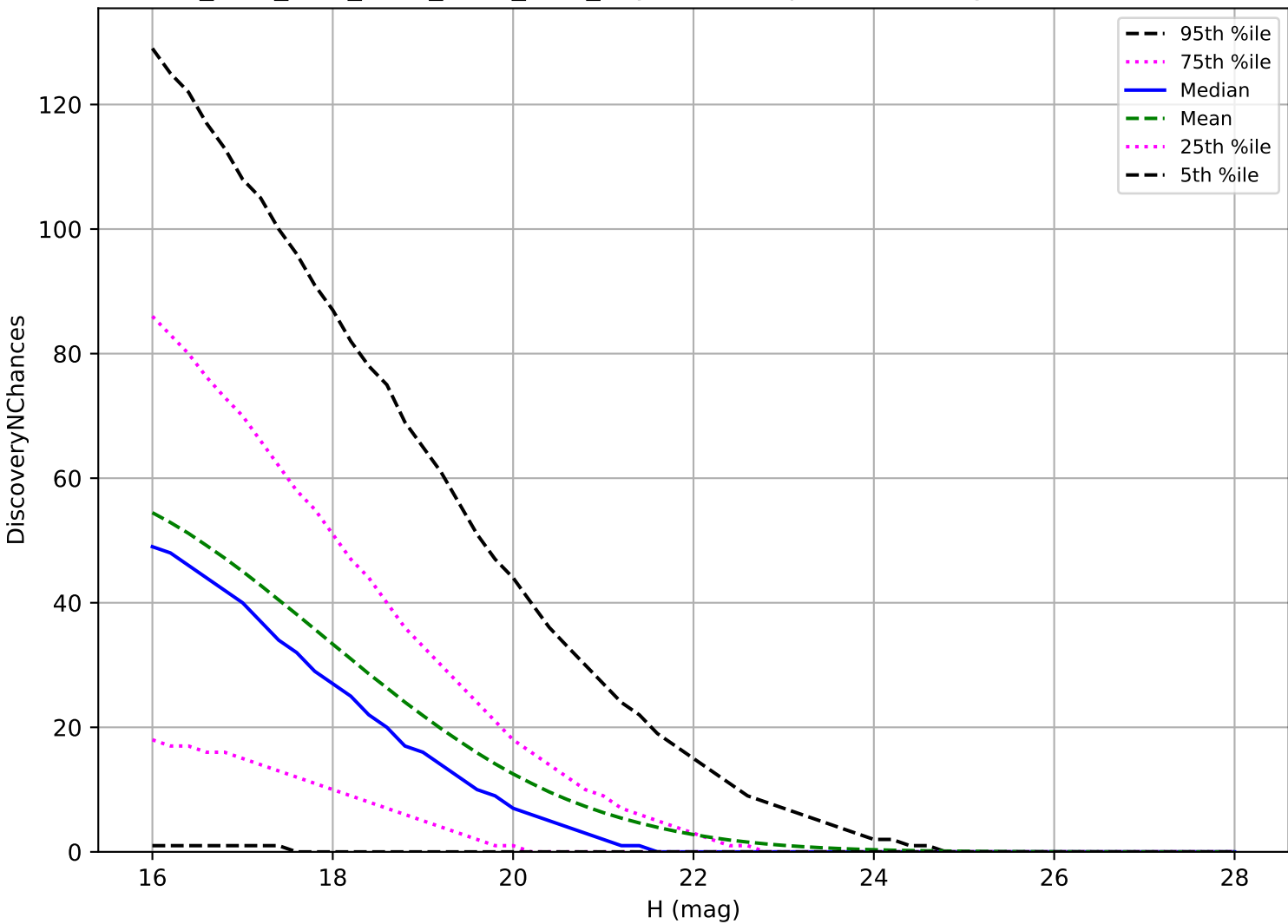
ddf_acor_sf15_lsf40_lsr50_v3.4_10yrs: PHA 3 pairs in 15 nights detection loss
