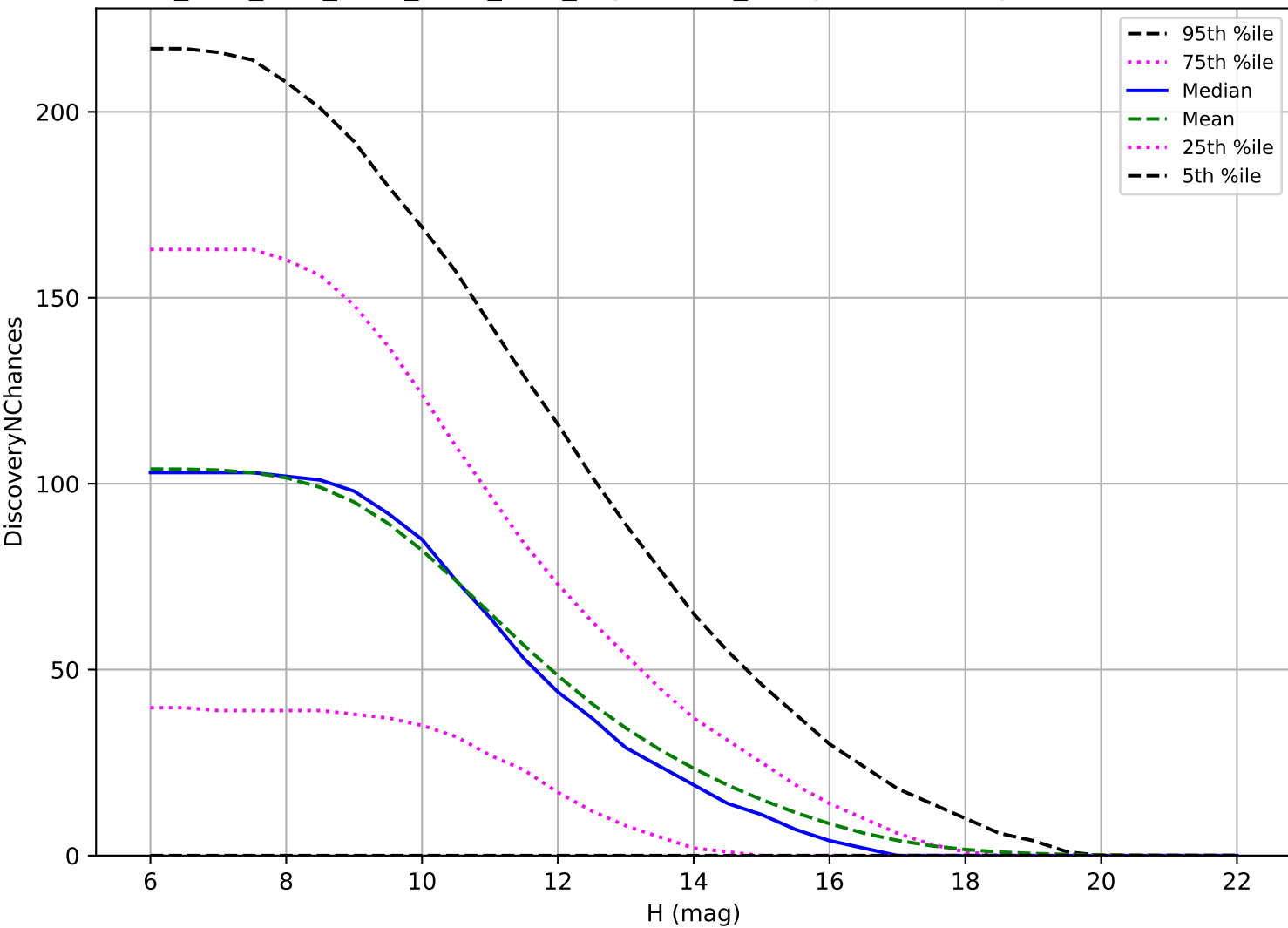
ddf_acor_sf15_lsf40_lsr50_v3.4_10yrs: OCC_r5 3 pairs in 15 nights detection loss
