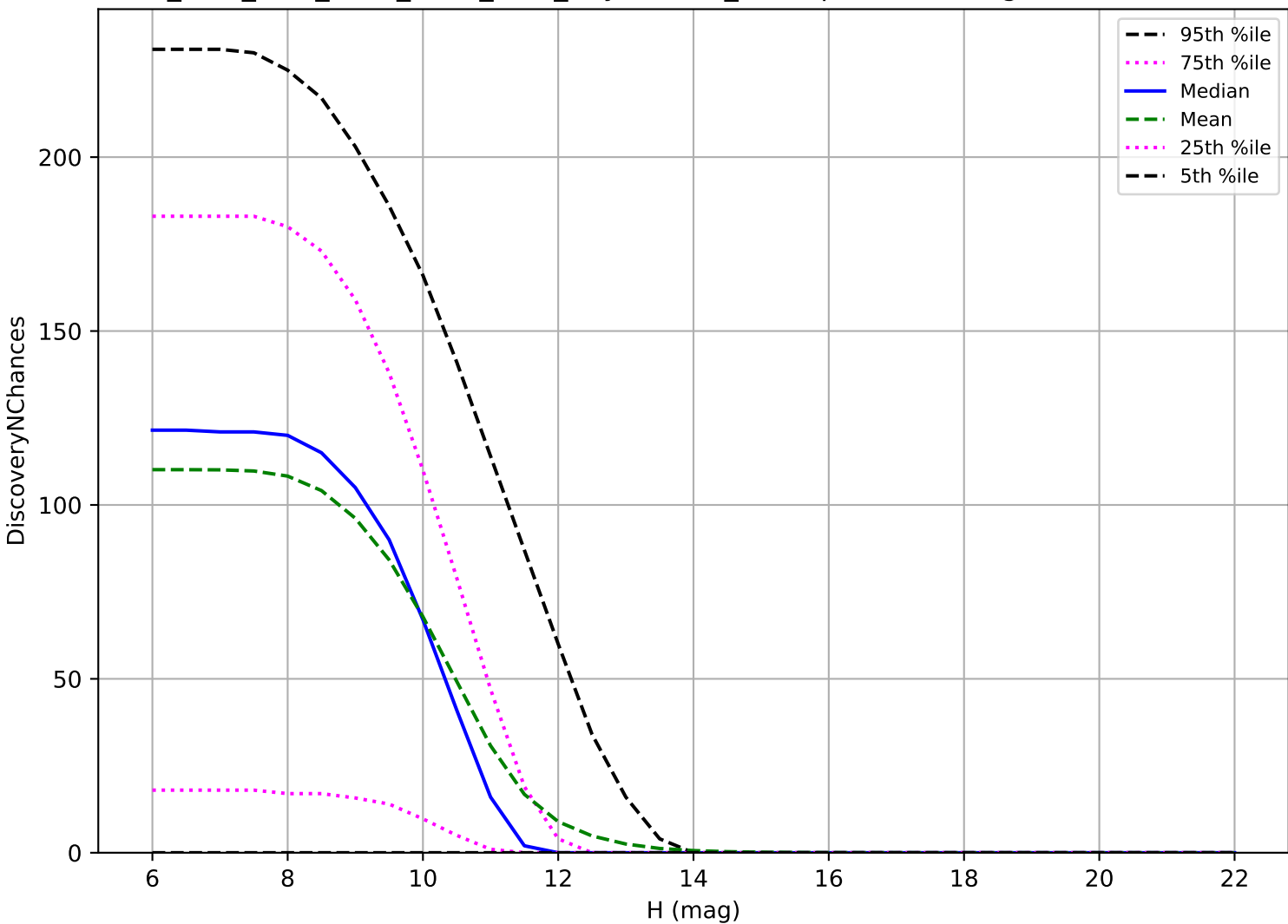
ddf_acor_sf15_lsf40_lsr50_v3.4_10yrs: OCC_r20 3 pairs in 15 nights detection loss
