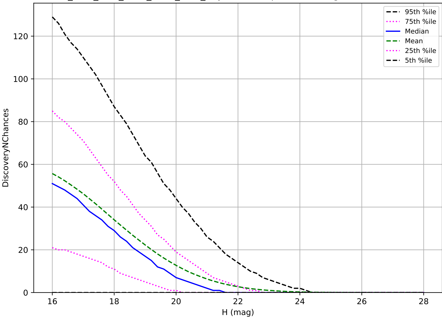
ddf_acor_sf15_lsf40_lsr50_v3.4_10yrs: NEO 3 pairs in 15 nights detection loss
