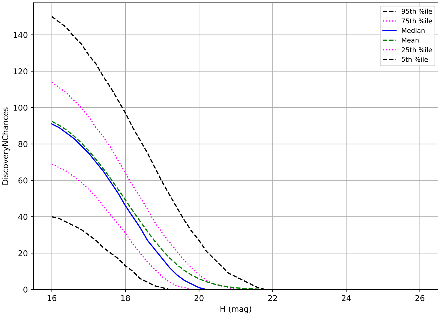
ddf_acor_sf15_lsf40_lsr50_v3.4_10yrs: MBA 3 pairs in 15 nights detection loss
