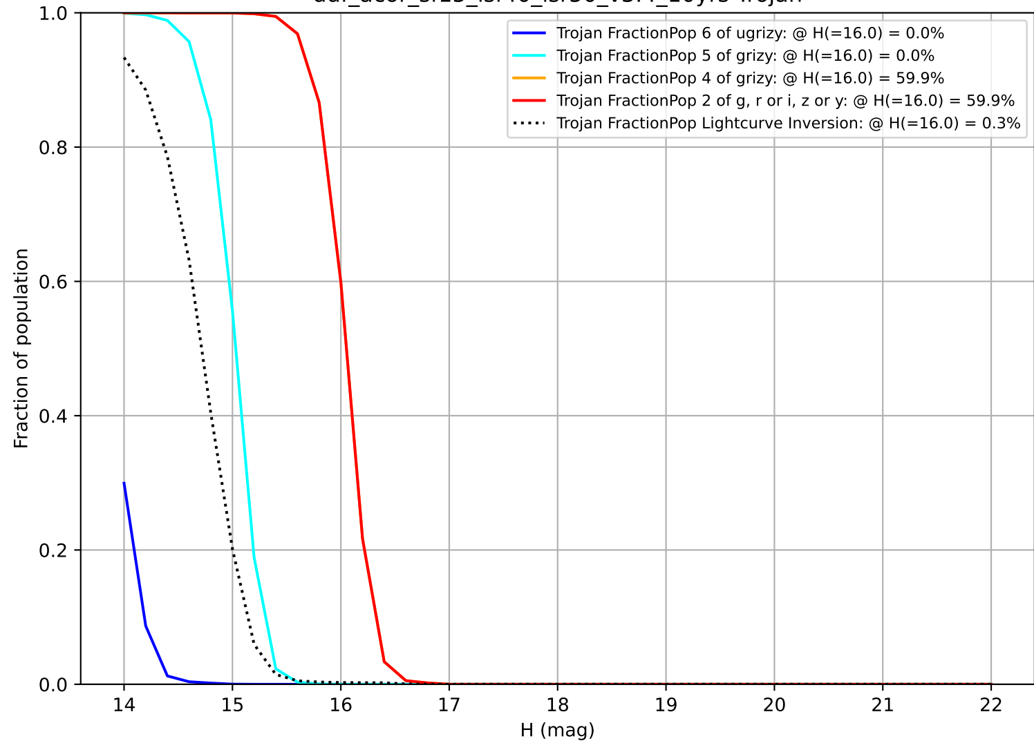
ddf_acor_sf15_lsf40_lsr50_v3.4_10yrs Trojan
