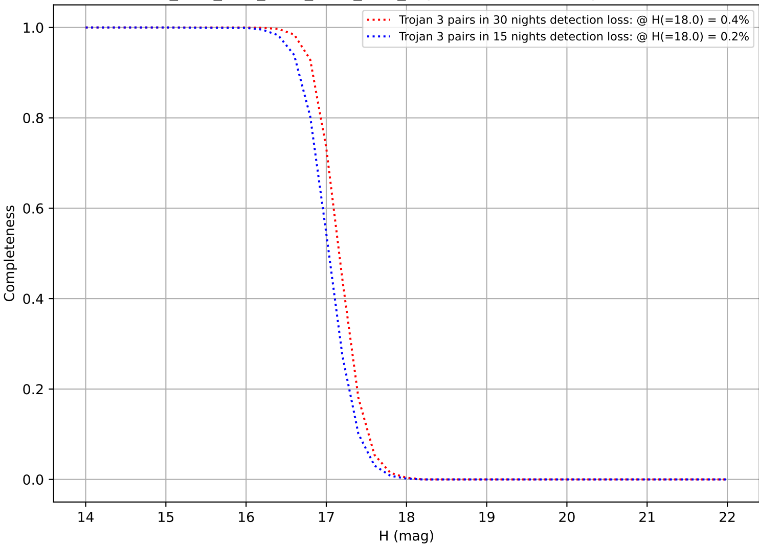
ddf_acor_sf15_lsf40_lsr50_v3.4_10yrs: DifferentialCompleteness
