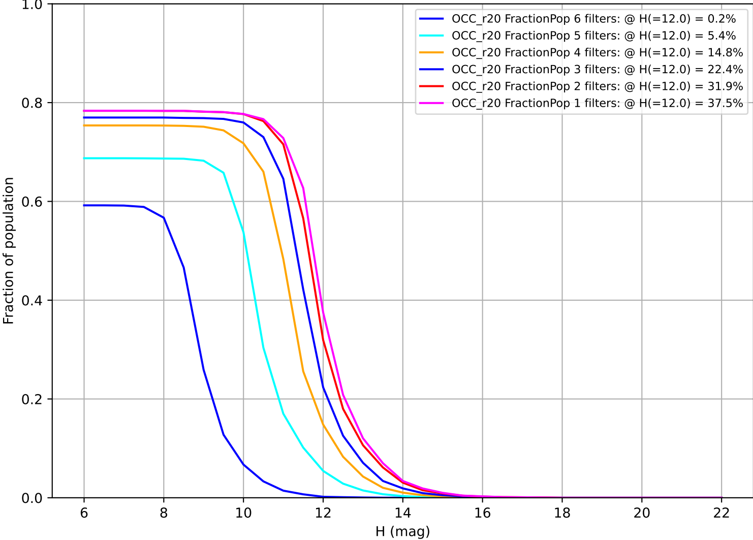
ddf_acor_sf15_lsf40_lsr50_v3.4_10yrs: Fraction of population with colors in X filters OCC_r20
